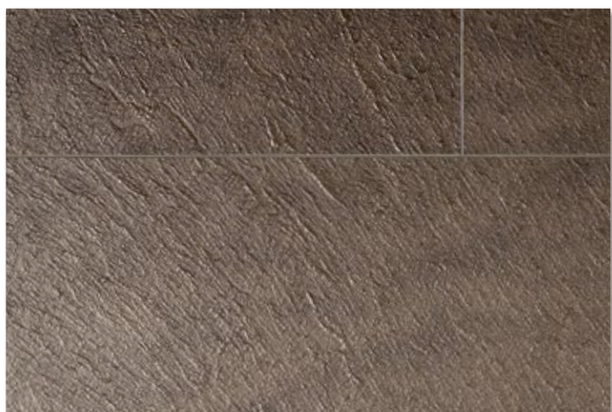
Schiefer Lias
