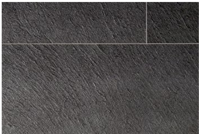
Schiefer Dinan
